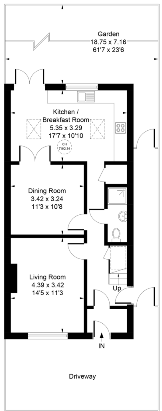
Ground Floor
