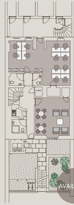
BASEMENT LAYOUT - 1:100
