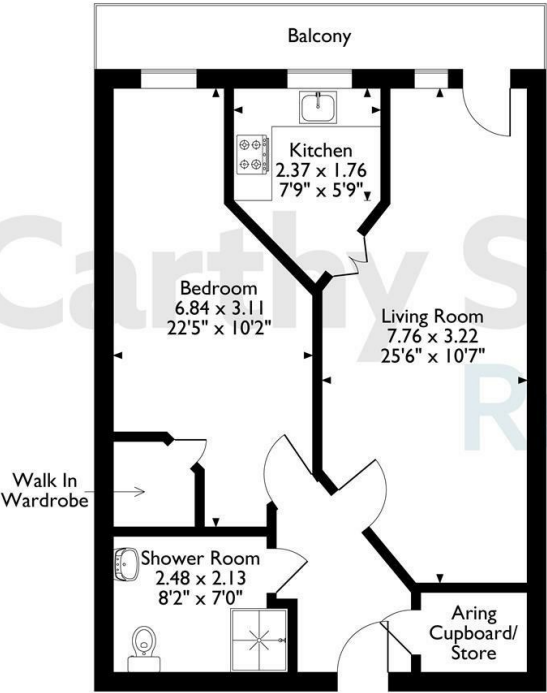
Second Floor Flat The position & size of doors, windows, appliances and other features are approximate only. © ehous. Unauthorised reproduction prohibited. Drawing ref. dig/8669055/DST.
