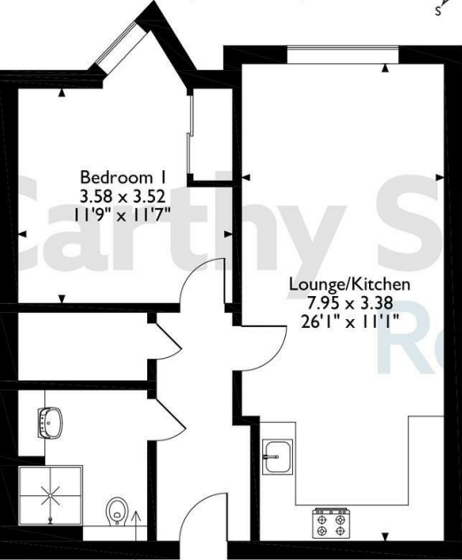
Shower Room 2.52 x 2.16 8'3" x 7'1" Ground Floor The position & size of doors, windows, appliances and other features are approximate only. © ehouse. Unauthorised reproduction prohibited. Drawing ref. dig/8667944/DST.
