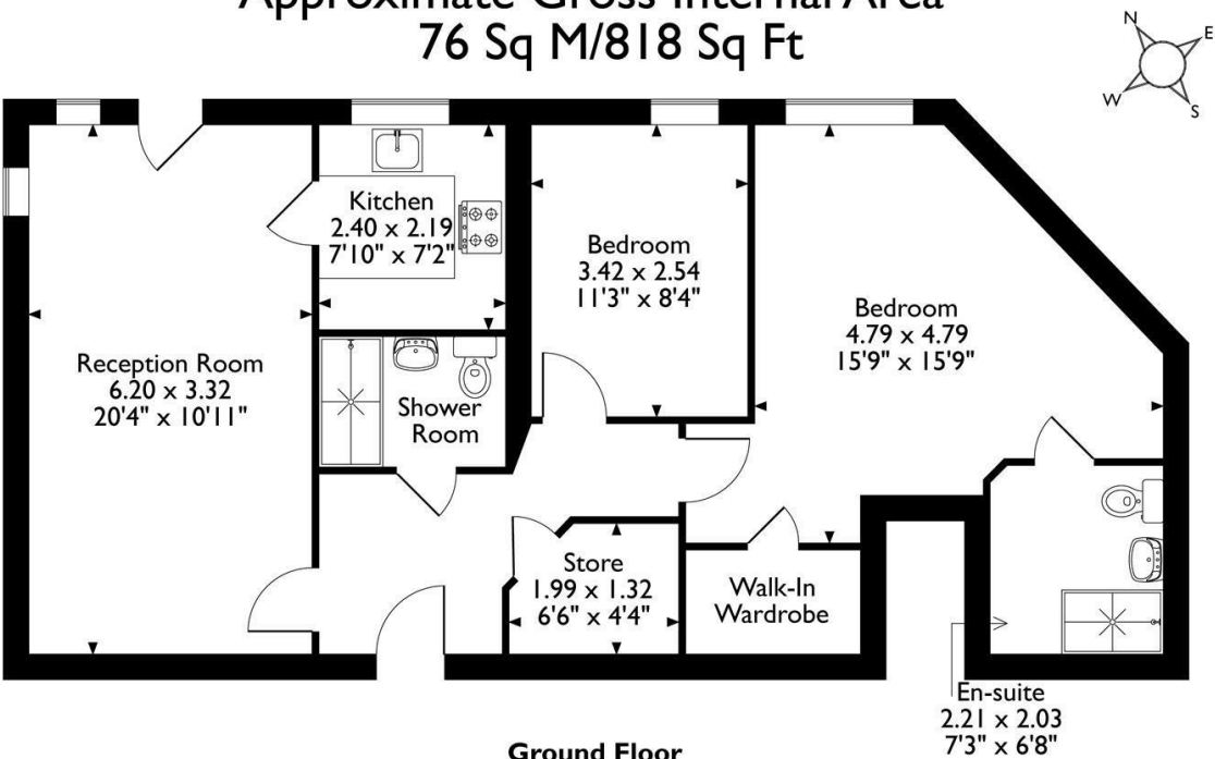
Ground Floor
