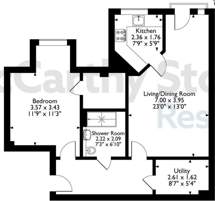
Third Floor The position & size of doors, windows, appliances and other features are approximate only. © ehous. Unauthorised reproduction prohibited. Drawing ref. dig/8668094/DST.
