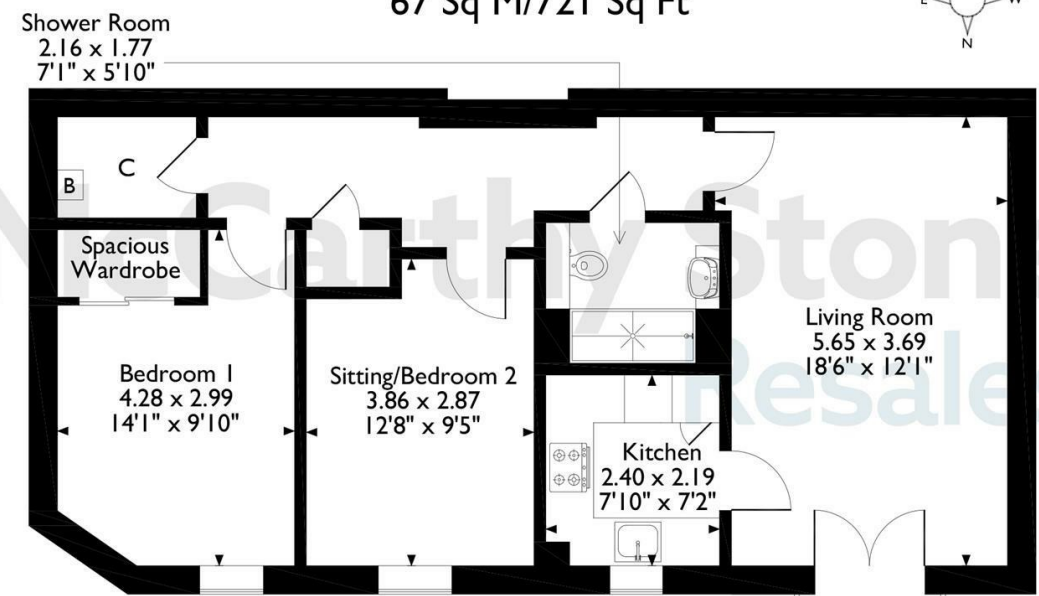
Forth Floor
