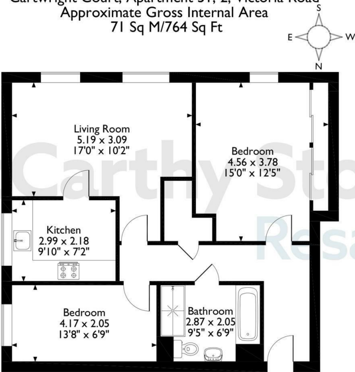
Fourth Floor
