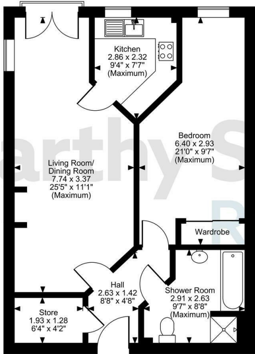
27 Dutton Court, Station Approach, Cheadle Hulme Approximate Gross Internal Area 642 Sq Ft/60 Sq M
