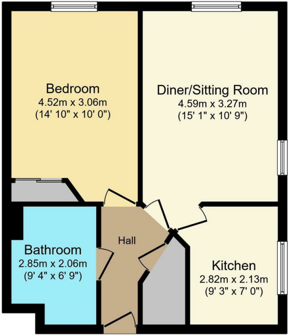
Floor Plan
