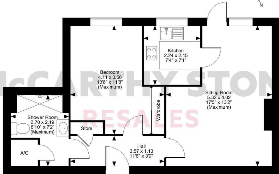
Second Floor
