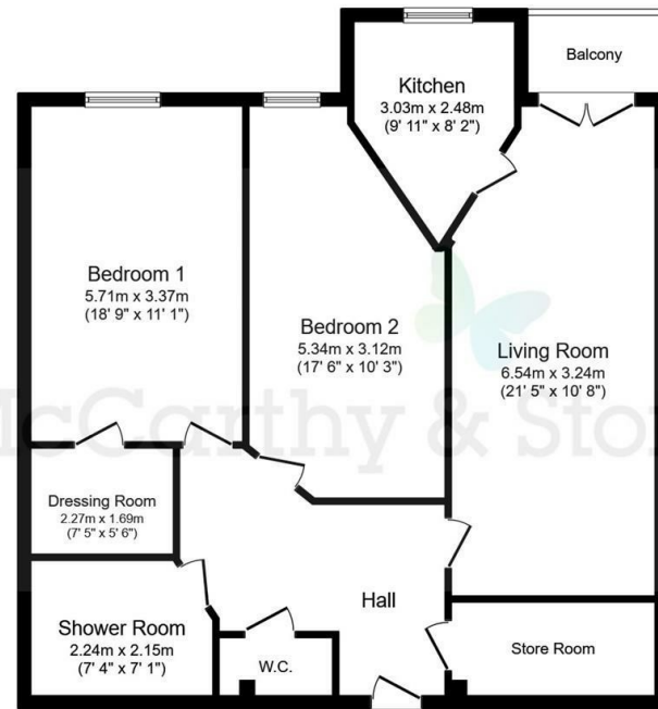
Floor Plan
