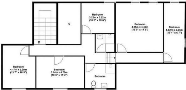
First Floor Approx 138.00 Sq meters (1485.00 Sq feet).
