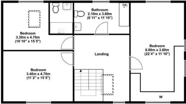
First Floor Approx 83.00 Sq meters (893.00 Sq feet).
