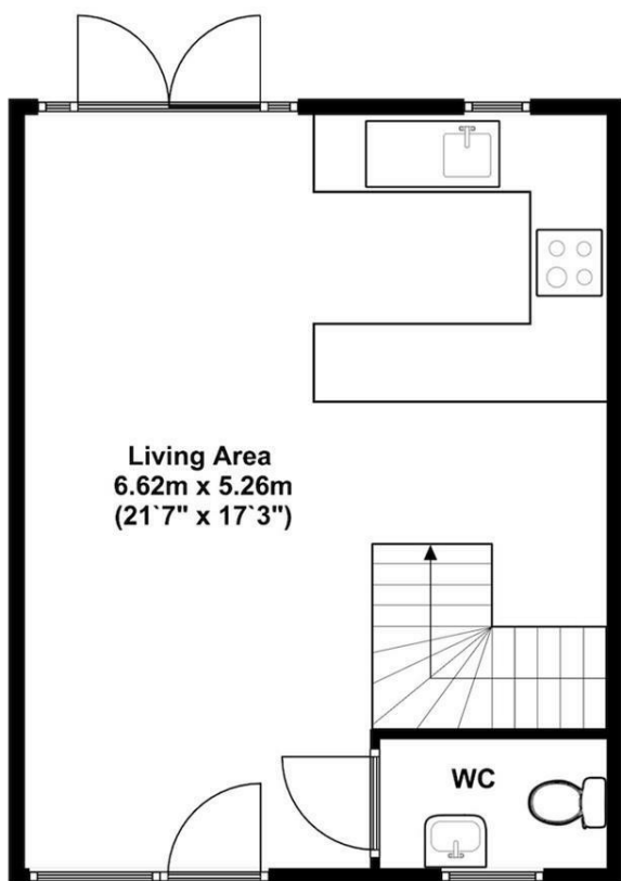
Ground Floor Approx 35.00 Sq meters (377.00 Sq feet).
