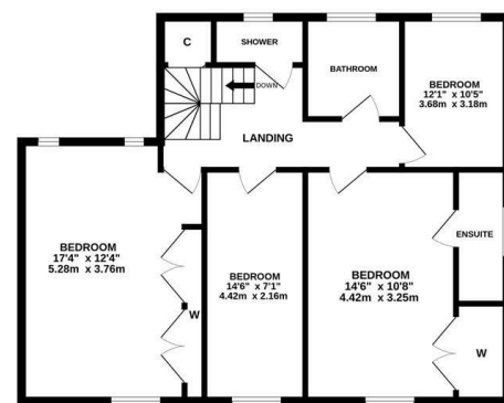
1ST FLOOR 768 sq.ft. (71.3 sq.m.) approx.
