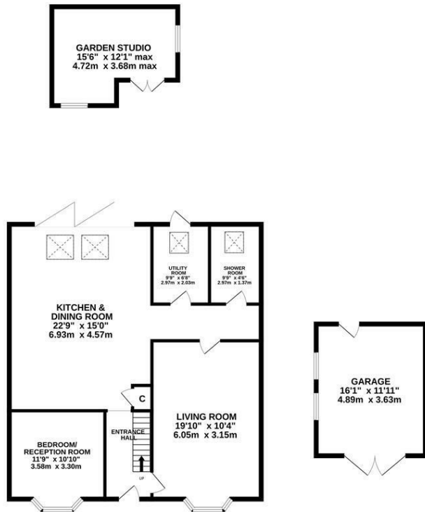
GROUND FLOOR 1420 sq.ft. (131.9 sq.m.) approx.
