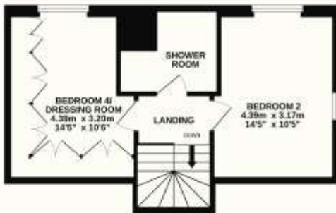
2ND FLOOR 38.5 sq.m. (414 sq.ft.) approx.
