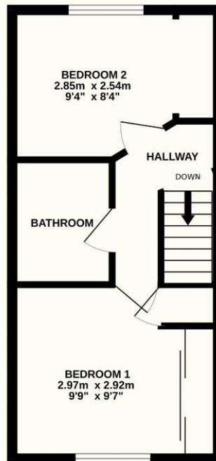
1ST FLOOR 28.0 sq.m. (302 sq.ft.) approx.
