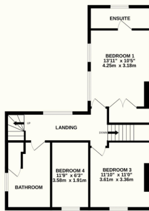
1ST FLOOR 650 sq.ft. (60.4 sq.m.) approx.
