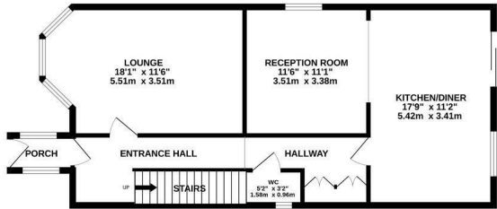
GROUND FLOOR 704 sq.ft. (65.4 sq.m.) approx.
