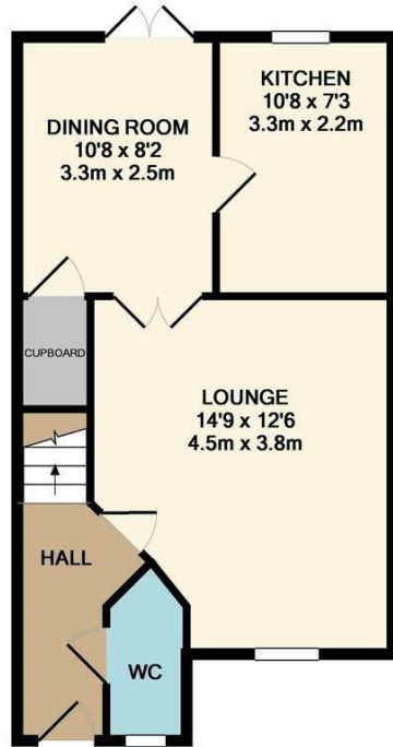
GROUND FLOOR APPROX. FLOOR AREA 419 SQ.FT. (38.9 SQ.M.)
