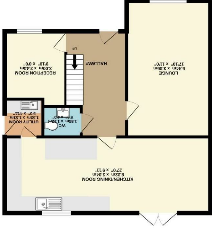
GROUND FLOOR 63.7 sq.m. (685 sq.ft.) approx.
