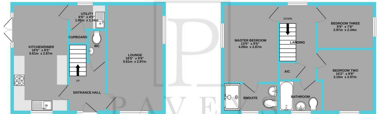
GROUND FLOOR 470 sq.ft. (43.7 sq.m.) approx.
