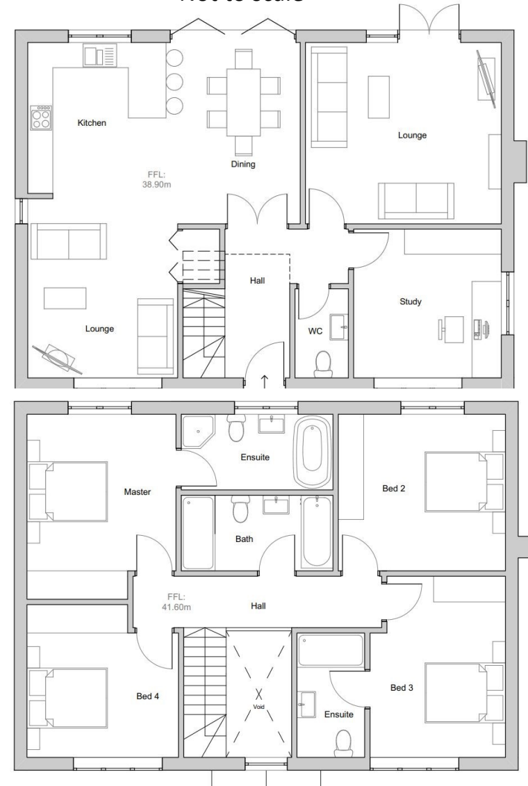
FLOORPLANS (Planning Illustration) Not to scale
