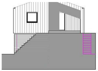
Proposed elevation to South [150]
