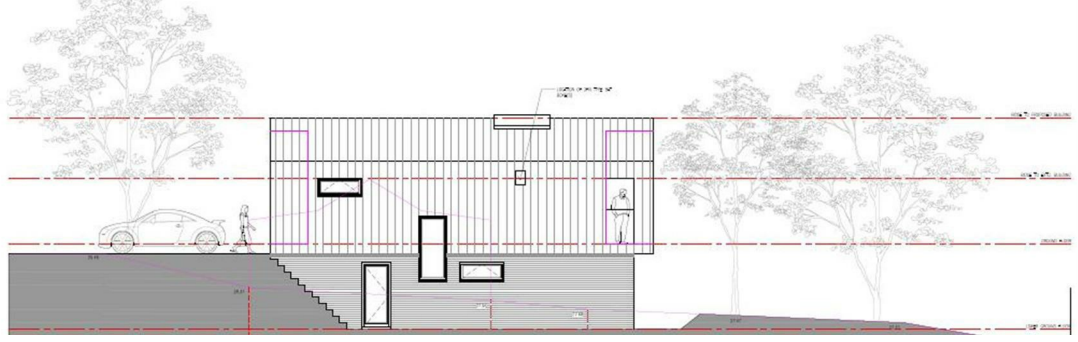
Proposed elevation to West [150]
