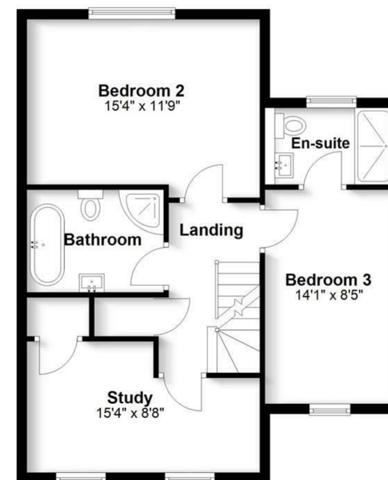
First Floor Approx. 628.4 sq. feet
