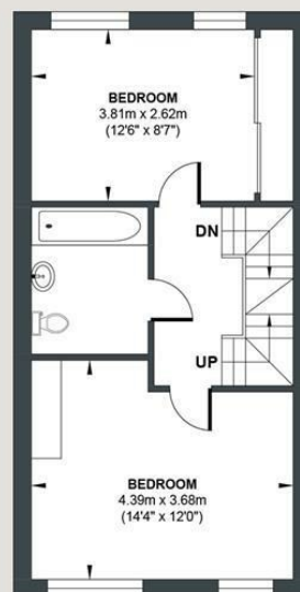
FIRST FLOOR Approximate Floor Area 437.12 sq ft (40.61 sq m)
