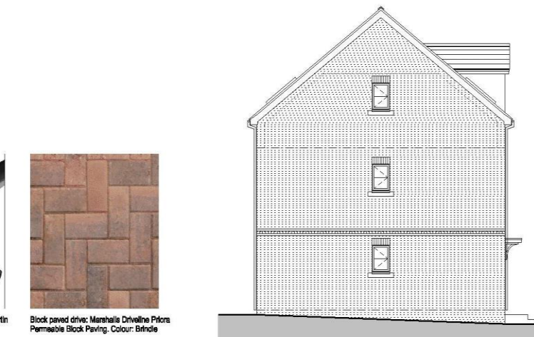
Gable (South) Elevations
