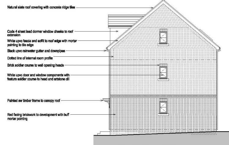
Gable (North) Elevations
