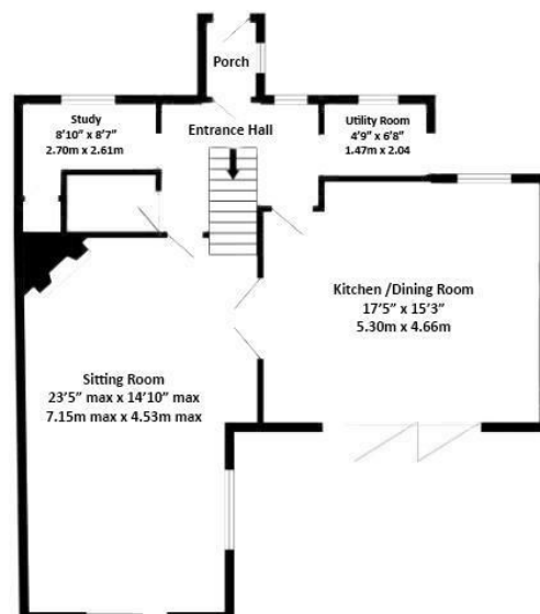
GROUND FLOOR 768 sq.ft. (71.4 sq.m.) approx.
