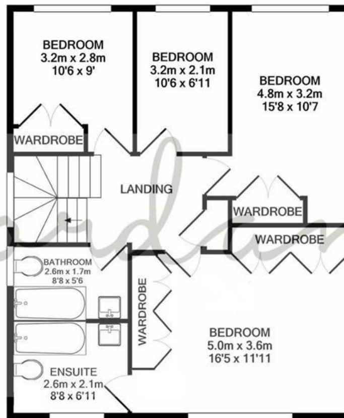
1ST FLOOR APPROX. FLOOR AREA 67.5 SQ.M. (727 SQ.FT.)
