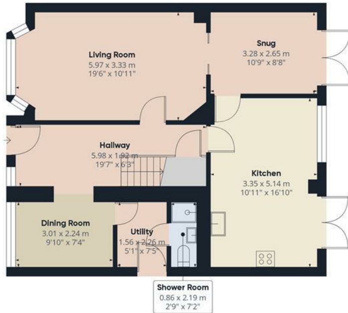
Floor 0 Building 1
