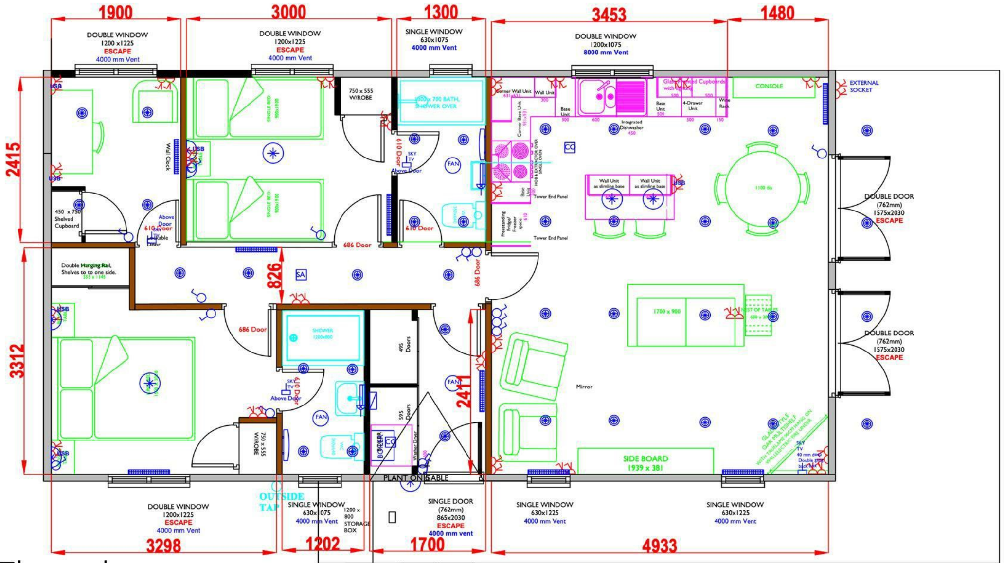
Floor plan 38' x 20' Nordic Lodge
