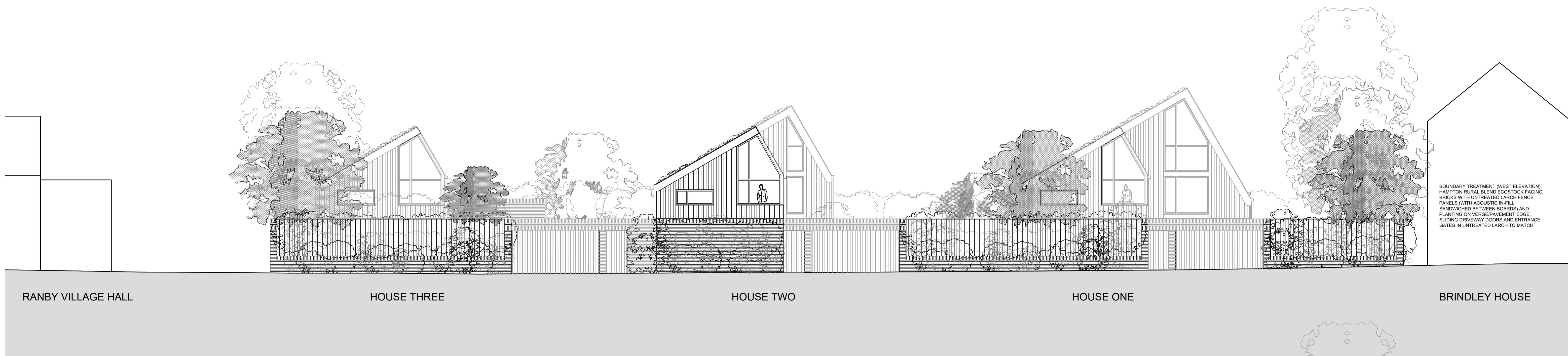
SITE SECTION Di-Di (BLYTH ROAD / WEST ELEVATION) AS PROPOSED
