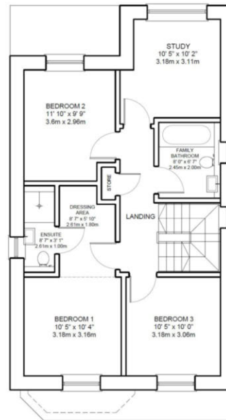
PLOT 05 First Floor Plan 812.6 sq.m / 75.5 sq.m
