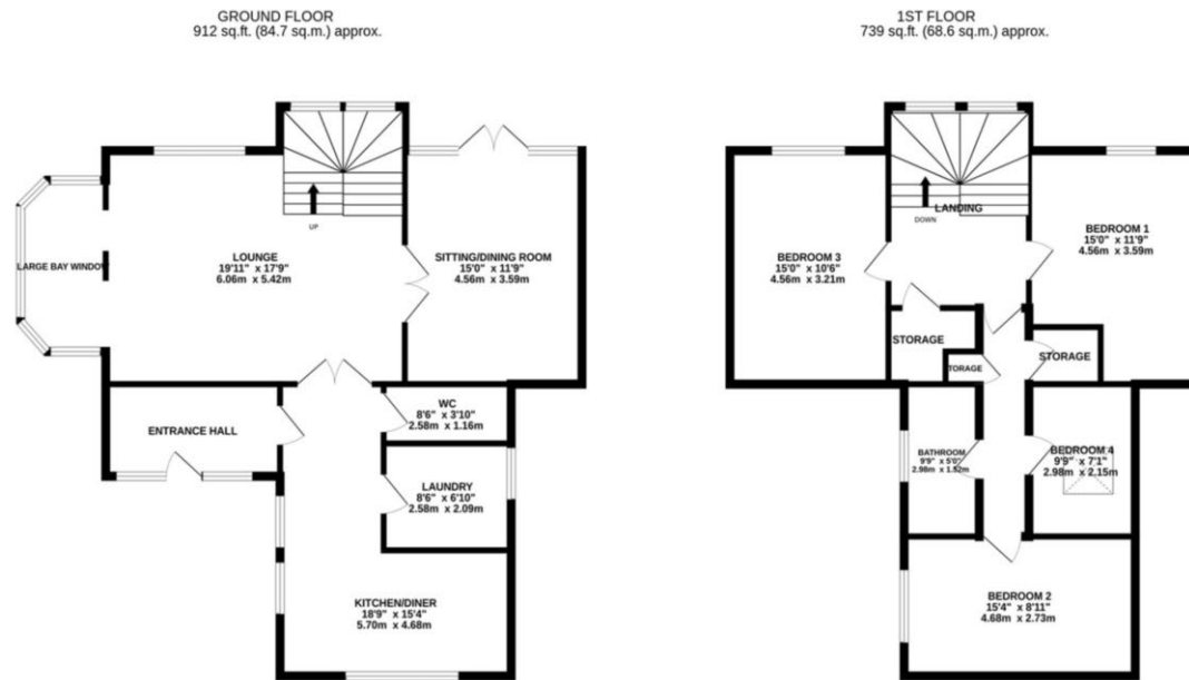
TOTAL FLOOR AREA: 1650 sq.ft. (153.3 sq.m.) approx. Measurements are approximate. Not to scale. Illustrative purposes only. Made with Metropix ©2024
