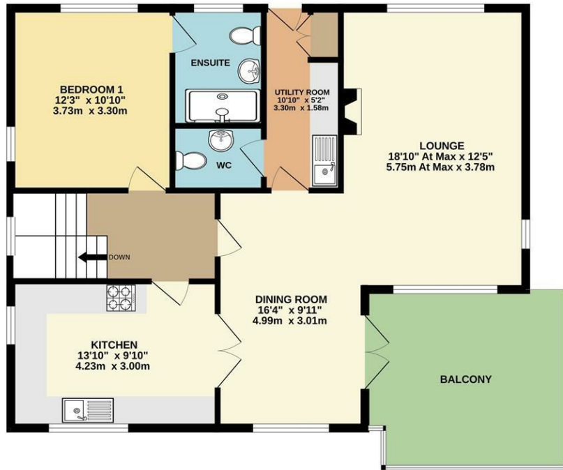
1ST FLOOR 869 sq.ft. (80.7 sq.m.) approx.
