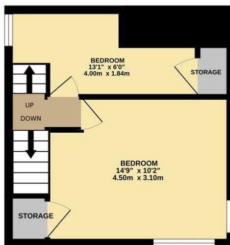
1ST FLOOR 232 sq.ft. (21.6 sq.m.) approx.
