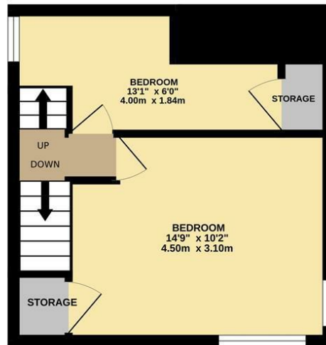
TOTAL FLOOR AREA : 742 sq.ft. (69.0 sq.m.) approx.
