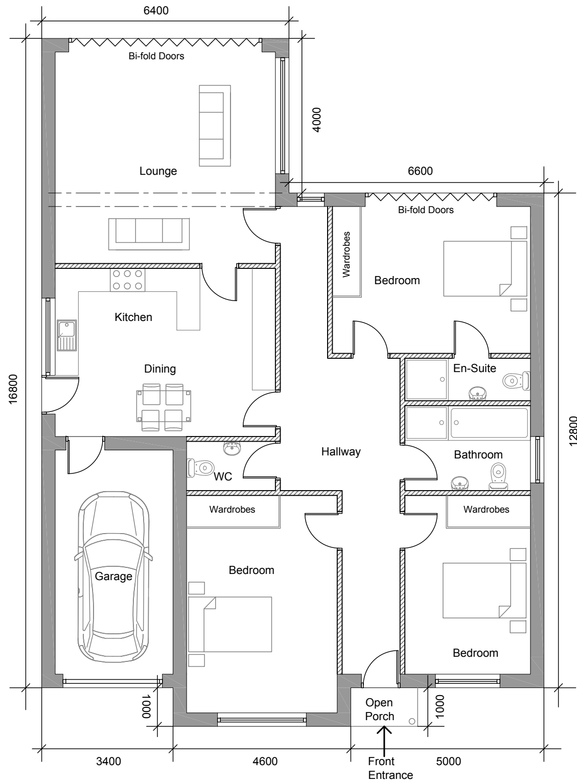
DWELLING TYPE A -FLOOR PLAN ( 3 BEDROOM)
