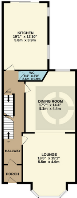
GROUND FLOOR 931 sq.ft. (86.5 sq.m.) approx.
