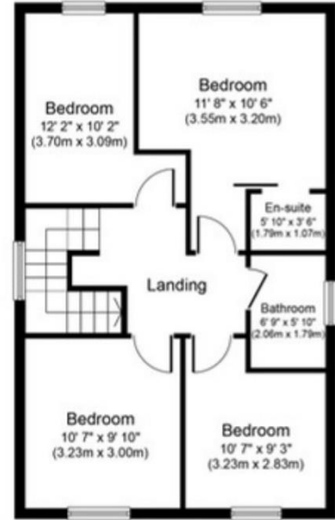
First Floor Approximate Floor Area 579 sq. ft. (53.8 sq. m.)
