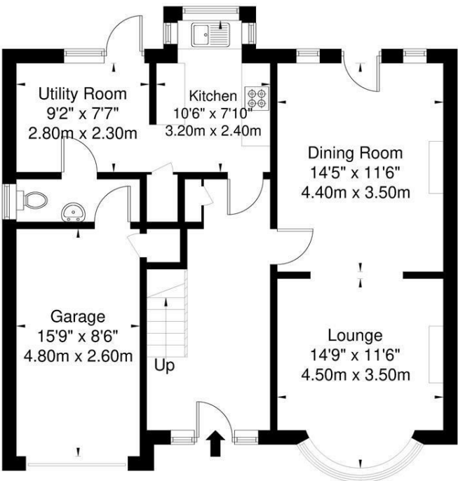
GROUND FLOOR 73.7 sq m / 793 sq ft
