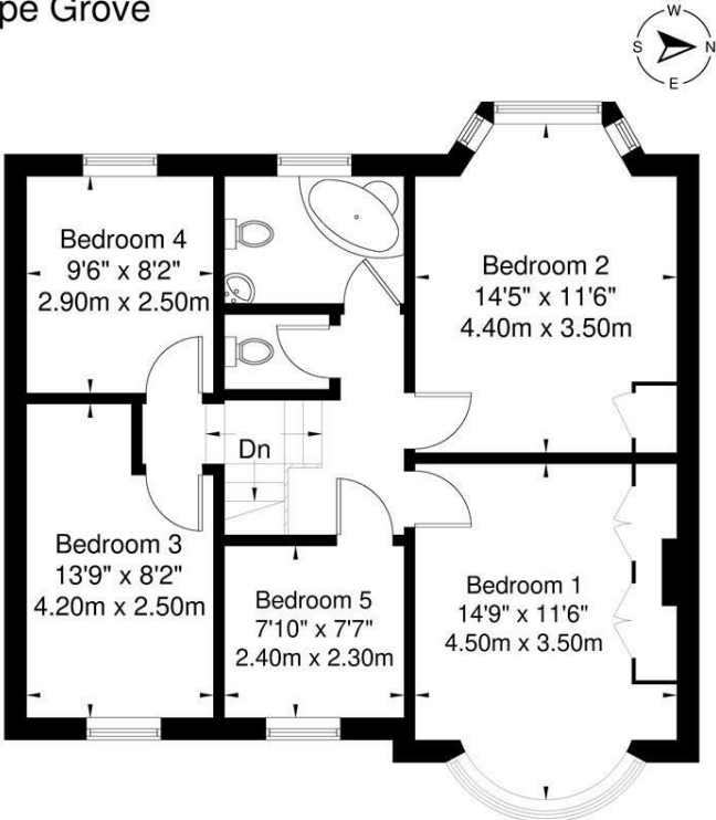
FIRST FLOOR 66.7 sq m / 717 sq ft
