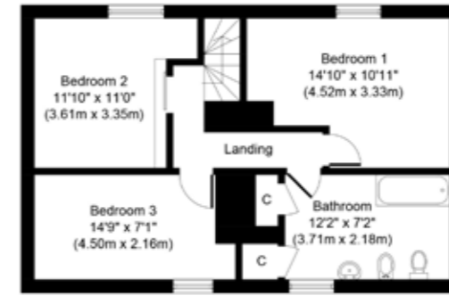
First Floor Approximate Floor Area 586 Sq. ft.
