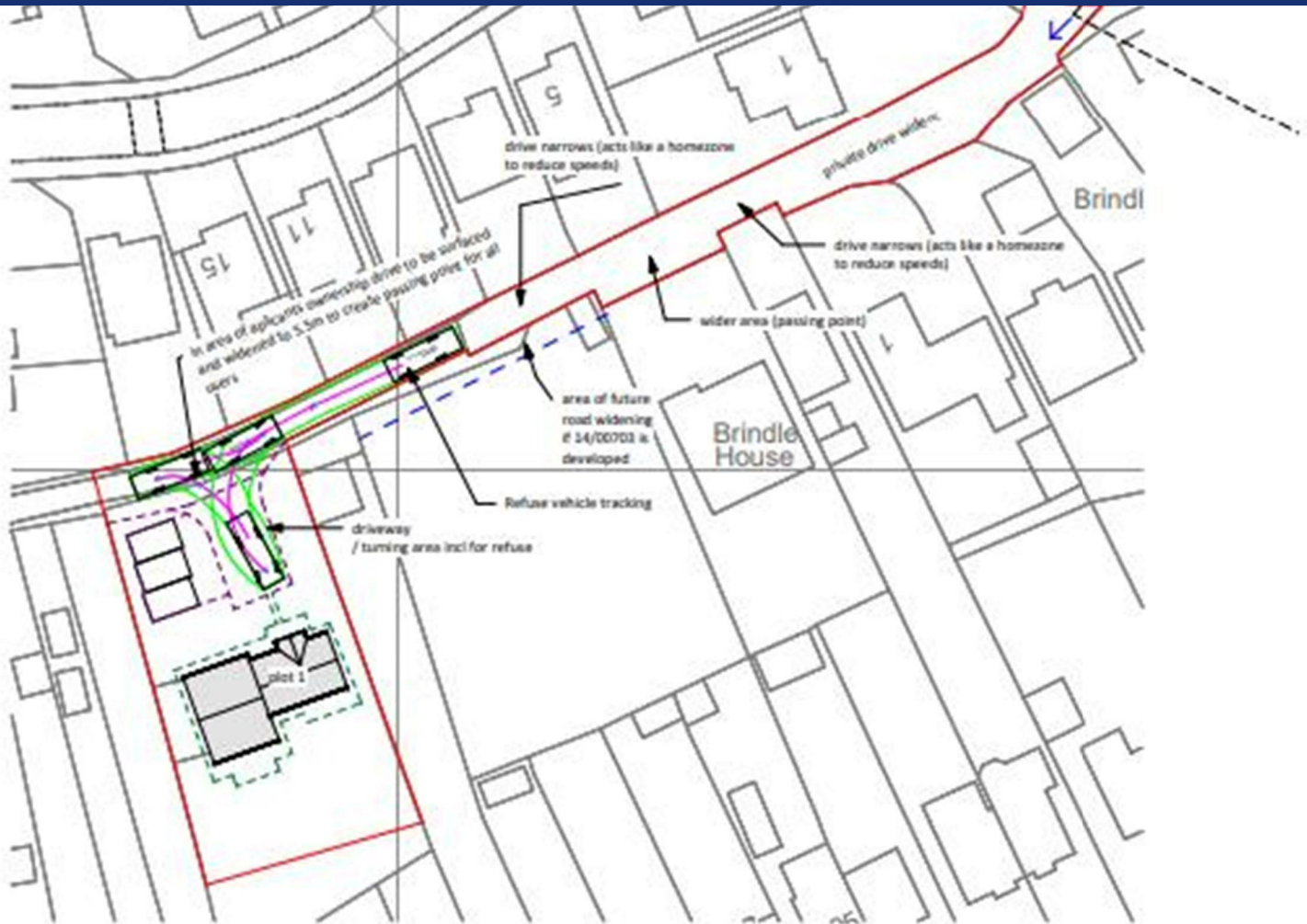
00 Site Plan - Proposed Widening / Turning
