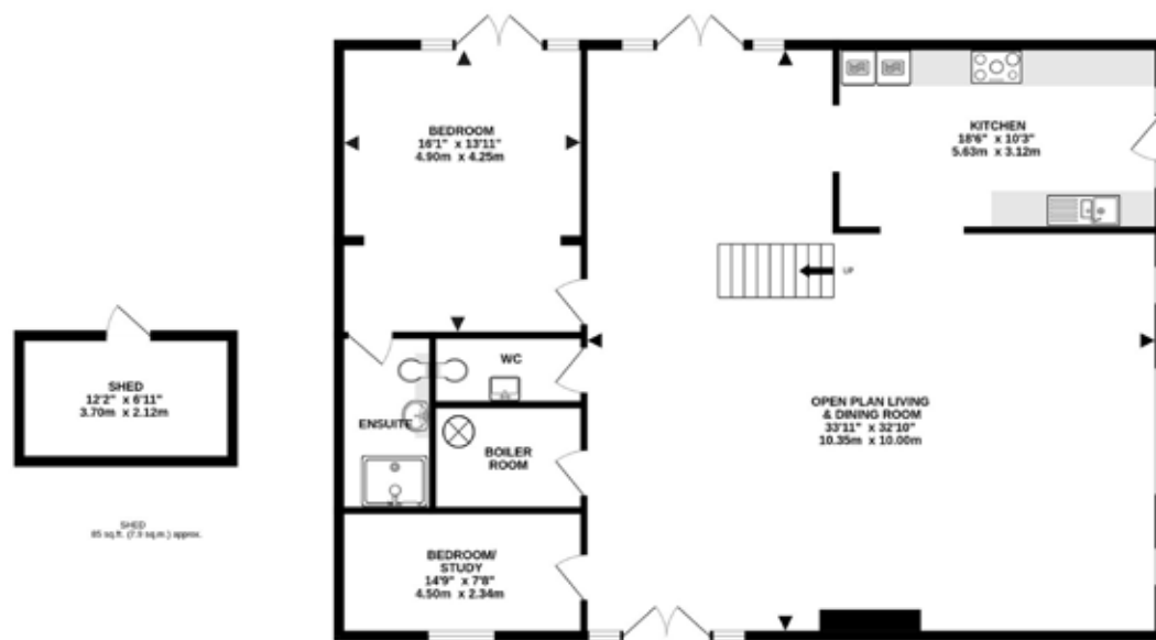
GROUND FLOOR 1529 sq.ft. (140.5 sq.m.) approx.
