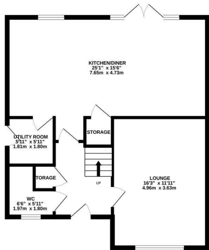
GROUND FLOOR 671 sq.ft. (62.4 sq.m.) approx.
