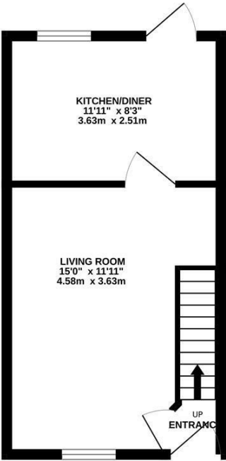
GROUND FLOOR 277 sq.ft. (25.7 sq.m.) approx.
