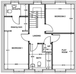
FIRST FLOOR LAYOUT
