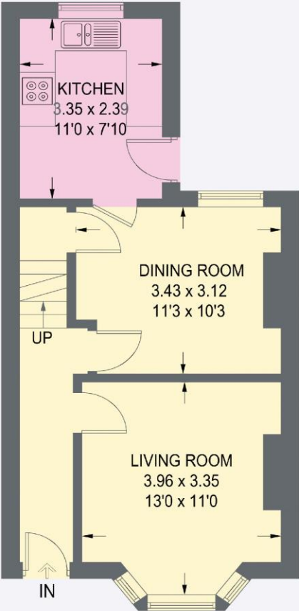
GROUND FLOOR 38.6 SQ M / 415 SQ FT
